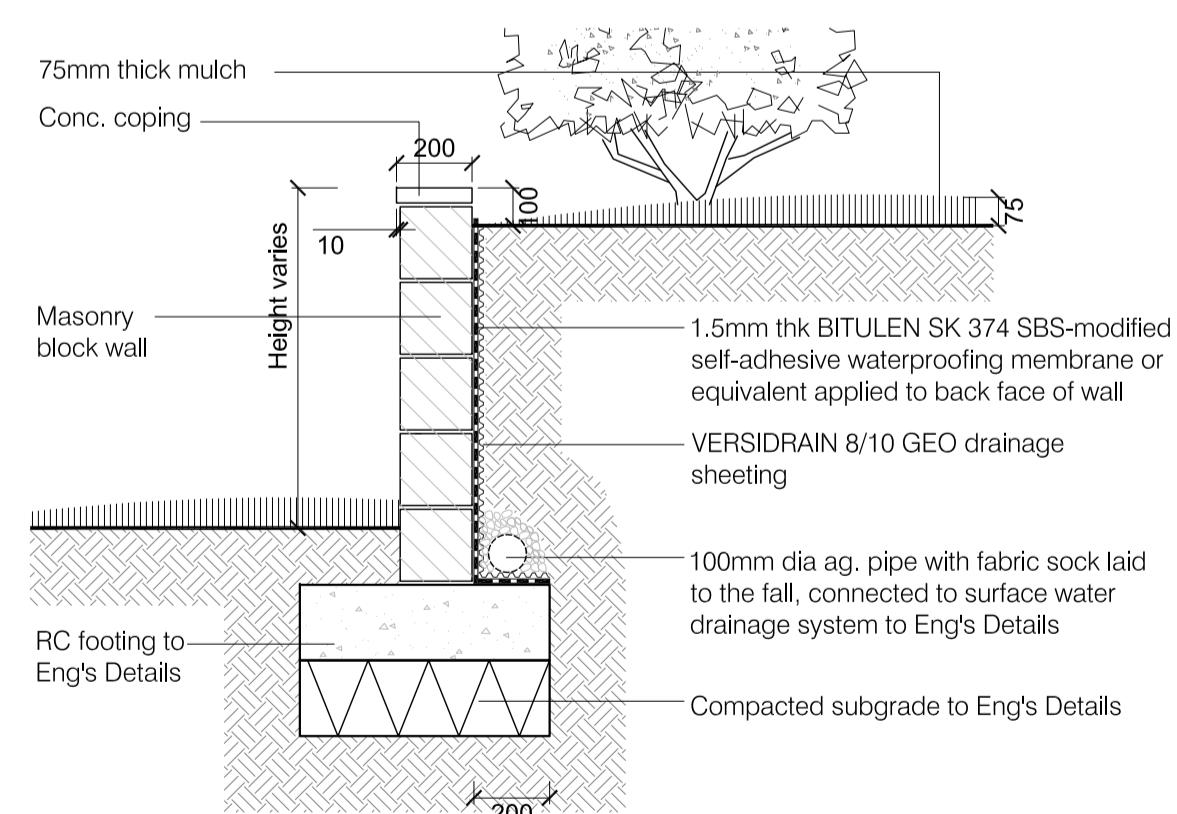
TYPICAL DETAIL 02: retaining wall scale: 1:20
